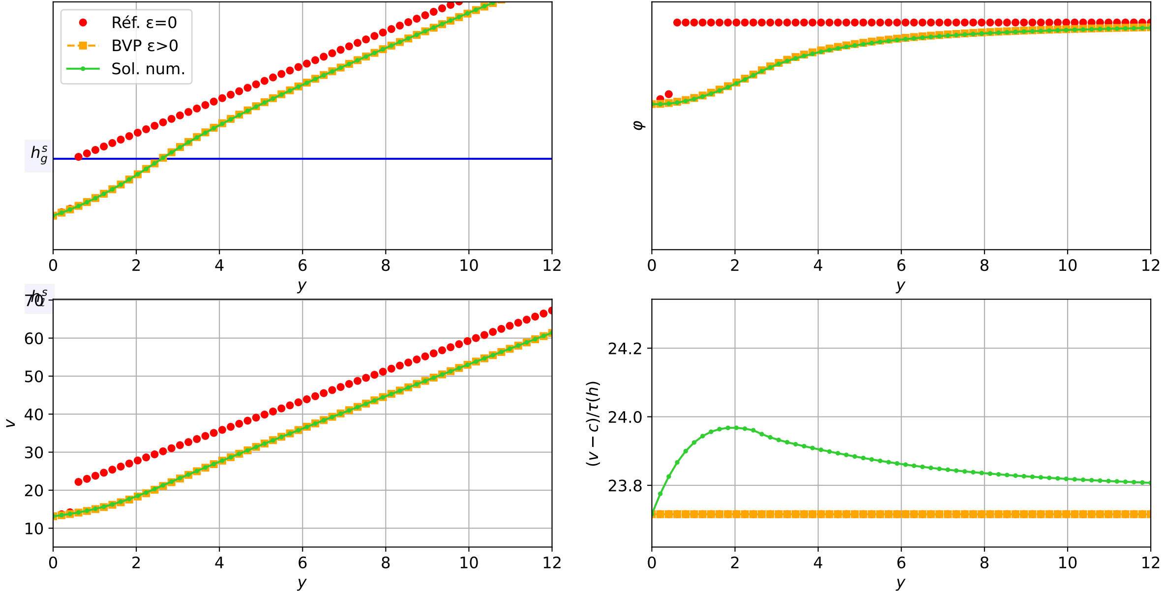
TEST-1_MG_TW : Validation TW | Travelling Wave (c=-2.0) | eps=1e-01 \varepsilon = 1e-01 , schéma implicite, N = 60 , dx = 0.2 dt = 3.02e-03 — t = 1.0012/4 (651 iter) — résidu eq. = 7.36e-06
